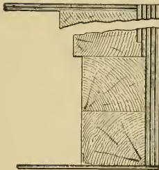
Side Armor Iron 3 to 5 in. Laminated.
